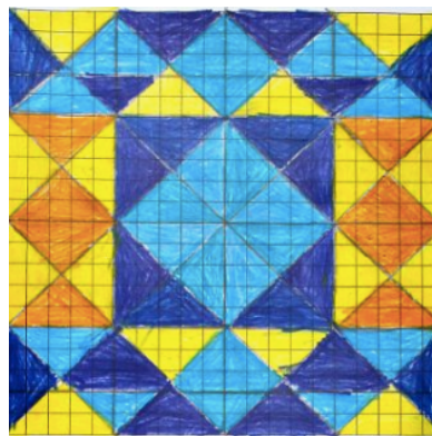
4. geometric patterns
